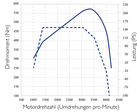
FICWG 136 PS Drehmoment/PS
