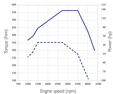
FIA e-VGT 160 HP Torque/Power curve
