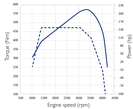
FIC WG 140 HP Torque/Power curve
